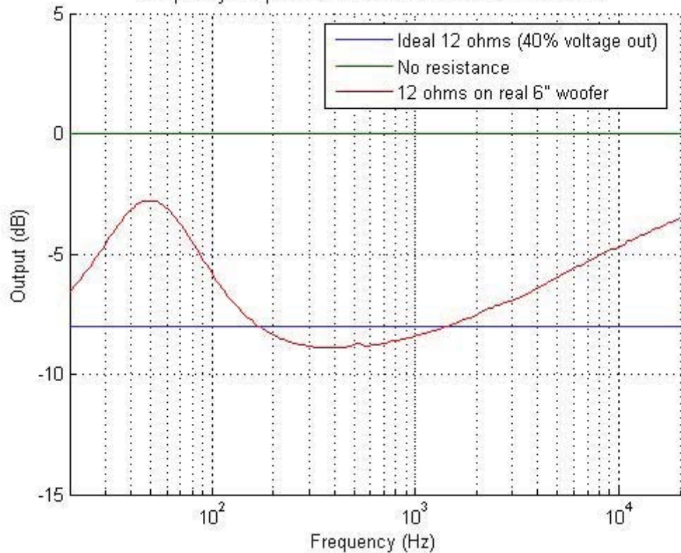
Frequency Response for Resistors in Series with 8 ohms
