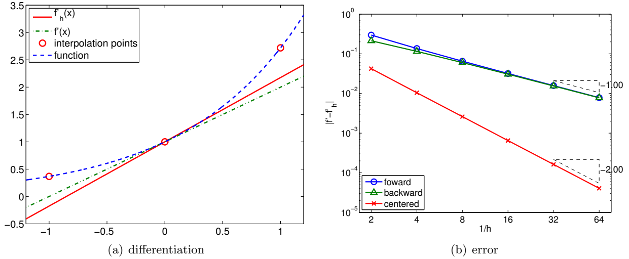
Figure 3.4: Centered difference.
