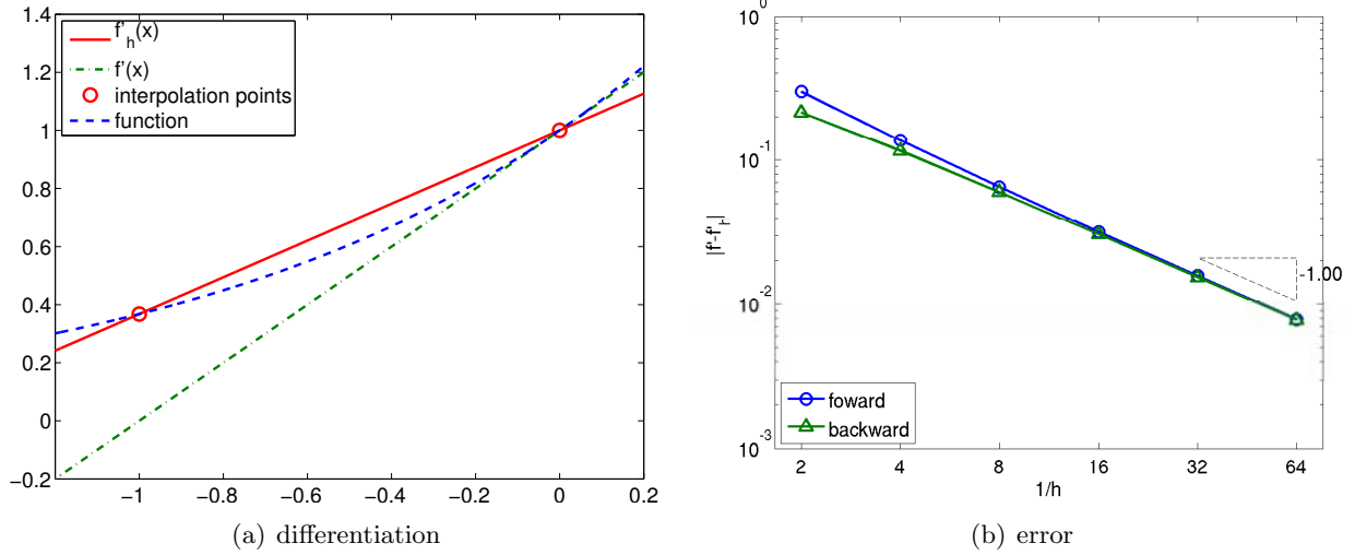
Figure 3.3: Backward difference.
