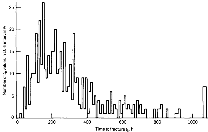
Histogram of lifetimes of 500 HDPE tubes subjected to 4 MPa at 80°C.
