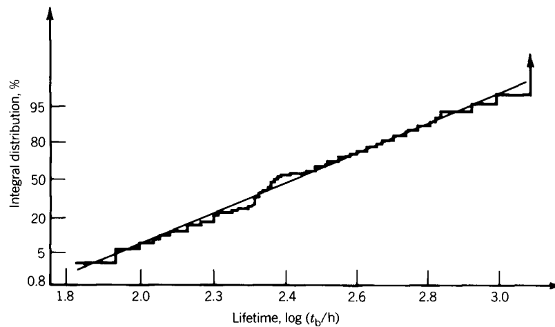
Log-normal cumulative probability plot.
