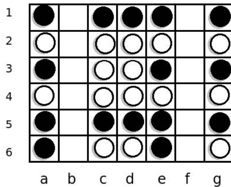
Courtesy of Victor Allis. Used with permission. Figure 4.3 in "A Knowledge-based Approach of Connect-Four. The Game is Solved: White Wins." Master's Thesis, Vrije University, 1988, pp. 26.
