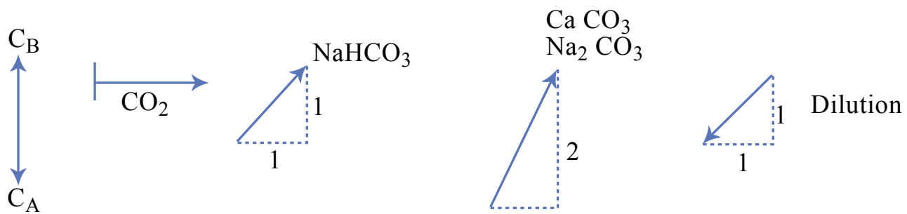
THE DEFFEYES DIAGRAM FOR 25°C
