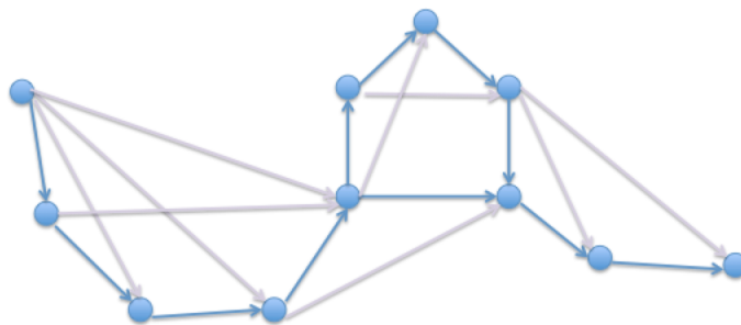
Figure 5.5: We can visualize the process of merging fragments into contigs by letting the nodes in a graph represent reads and edges represent overlaps. By removing the transitively inferable edges (the pink edges in this image), we are left with chains of reads ordered to form contigs.
