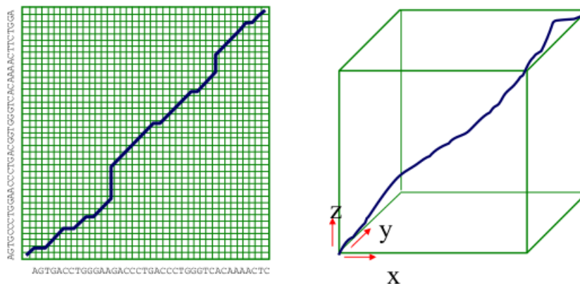
Figure 5.15: The Needleman-Wunsch algorithm for alignments of 2 and 3 genomes.
