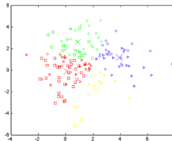
Figure 15.9: Examples of final cluster assignments of fuzzy k -means using k=4 with centroids, correct clusters, and most probable assigned clusters marked as crosses, shapes of points, and colors respectively. Note that the original data set is non-Gaussian.
