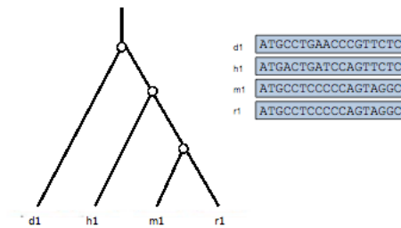
Figure 28.2: Gene Tree
