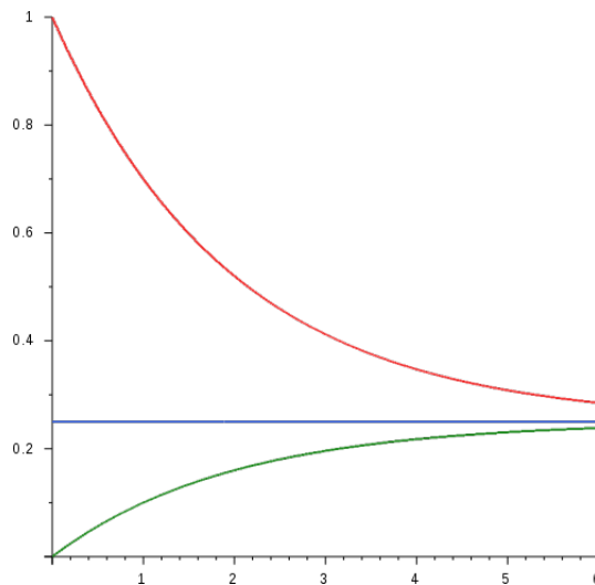
Figure 27.6: The y axis denotes probability of observing the bases - A(red), others(green). x axis denotes time.
