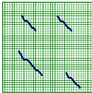
Figure 3.3: Local Alignment
