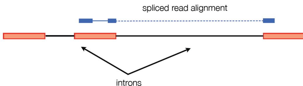
Figure 12.4: An example of a gap in alignment
