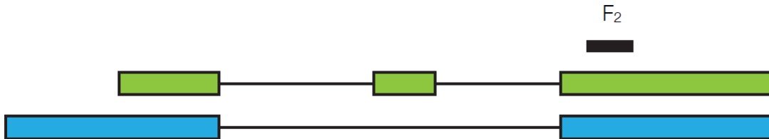
Figure 12.7: F_2
