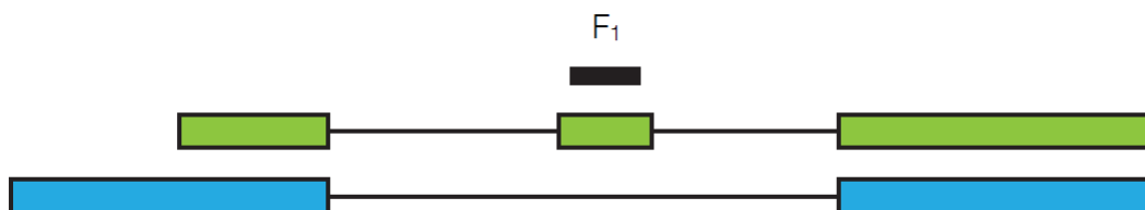
Figure 12.6: F_1
