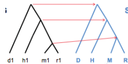
Figure 28.5: Mapping Diagram
