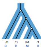
Figure 28.6: Nesting Diagram
