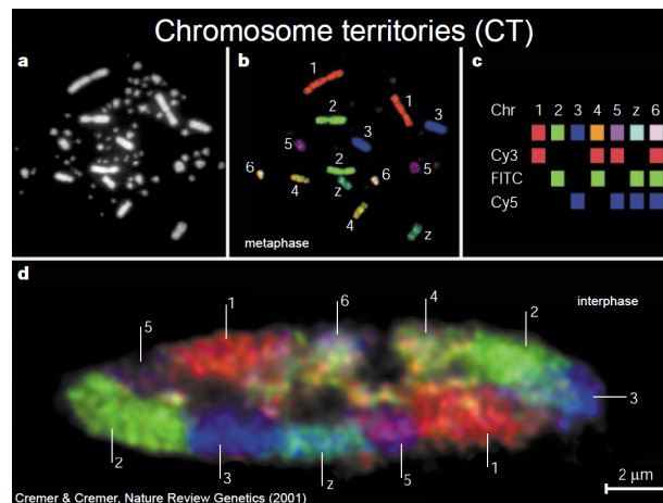
Figure 22.1: Chromosome Territories
