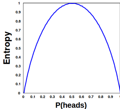
Figure 17.11: Entropy is maximized when both heads and tails have an equal chance of occurring
