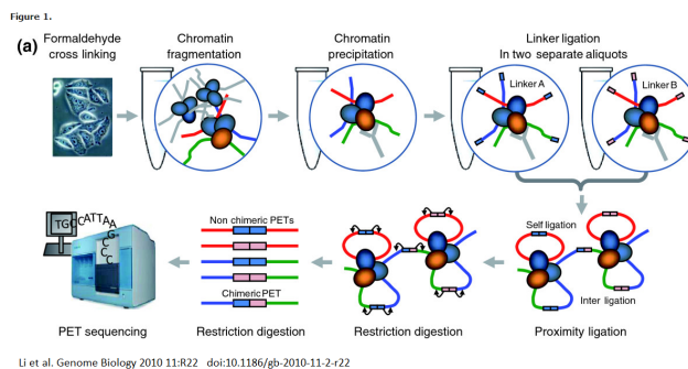
Figure 22.7: ChIA-PET protocol
