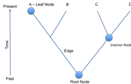
Figure 27.2: Defining tree terminology. A tree of branching nodes is depicted with leaves at the top and the root on the bottom. Time continues upward, toward the leaves.
