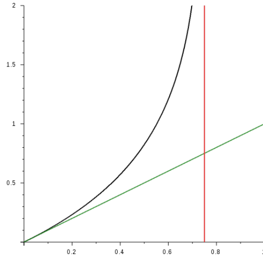
Figure 27.7: Fraction of altered bases (x axis) versus the Jukes Cantor distance(y axis). Black line denotes the curve, green is the trend line for small values of f while the red line denotes the asymptotic boundary.
