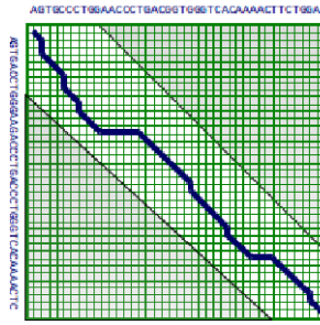
Figure 3.6: Bounded-space computation
