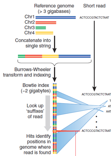
Figure 12.3: How Burrows-Wheeler indexing works
