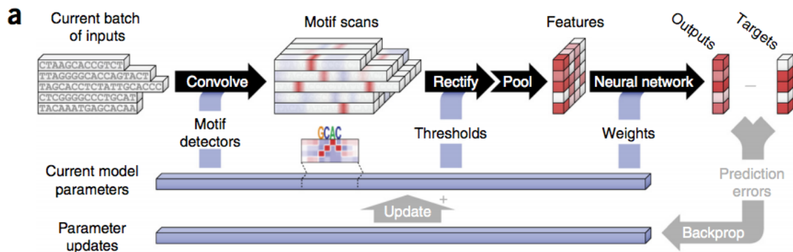
Figure 20.17: A flowchart of the DeepBind procedure (taken from the DeepBind paper). Five sequences are being processed in parallel by the model. The model convolves the sequences (we can think of the deepbind model as a filter scanning through the sequences), rectifies and pools them in order to produce a feature vector which is then passed through a deep neural network. The output from the deepnet is compared against the desired output and the error is back-propagated through the pipeline.
