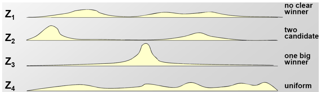
Figure 17.8: Examples of the Z matrix computed via EM, Gibbs Sampling, and the Greedy Algorithm
