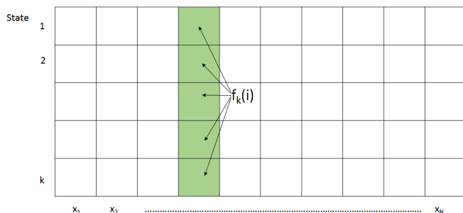
Figure 8.2: The Forward Algorithm
