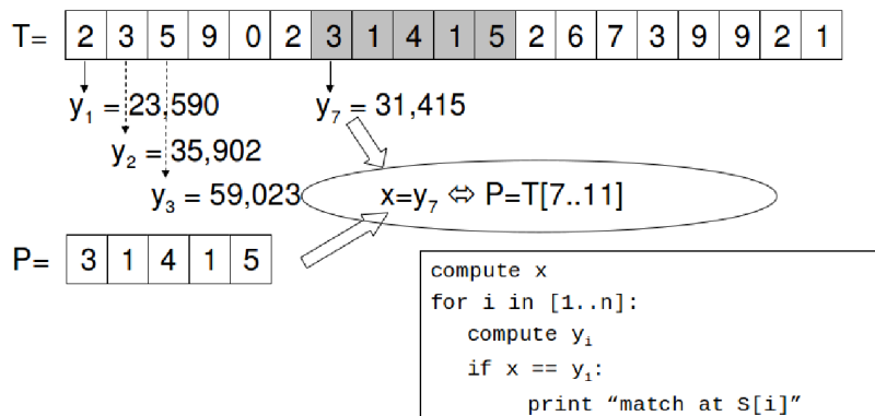
Figure 3.10: Naive Karp-Rabin algorithm
