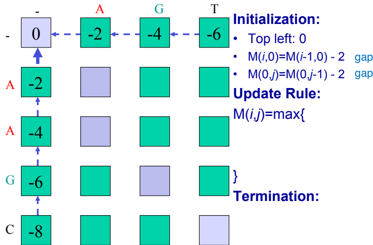
Figure 2.9: (Example) Initial setup for Needleman-Wunsch
