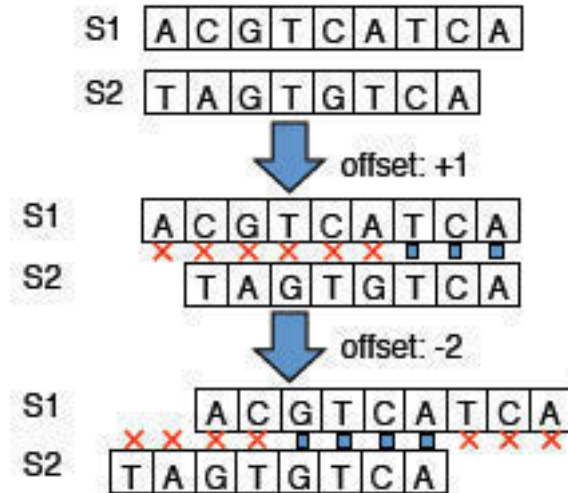
Figure 2.4: Example of longest common substring formulation
