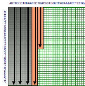
Figure 3.7: Linear-space computation for optimal alignment score
