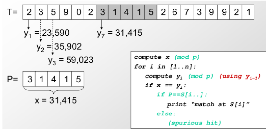
Figure 3.11: Final Karp-Rabin algorithm
