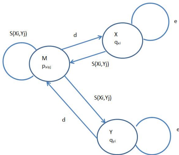
Figure 8.6: HMM model for alignment with affine gap penalties
