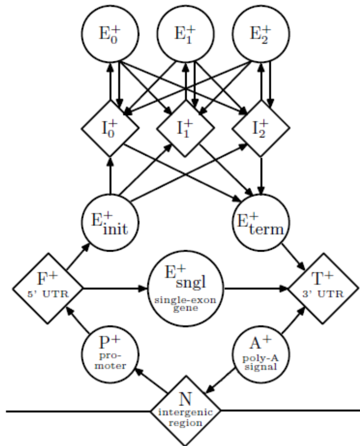
Figure 8.7: State Space Diagram used in GENSCAN
