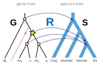
Figure 28.22: MPR reconciliation of genes and species tree.
