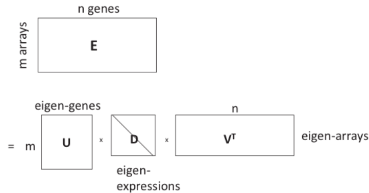
Figure 20.6: Eigen-gene decomposition using PCA
