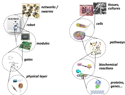
Figure 26.1: The layers of abstraction in robotics compared with those in biology (credit to Ron Weiss).
