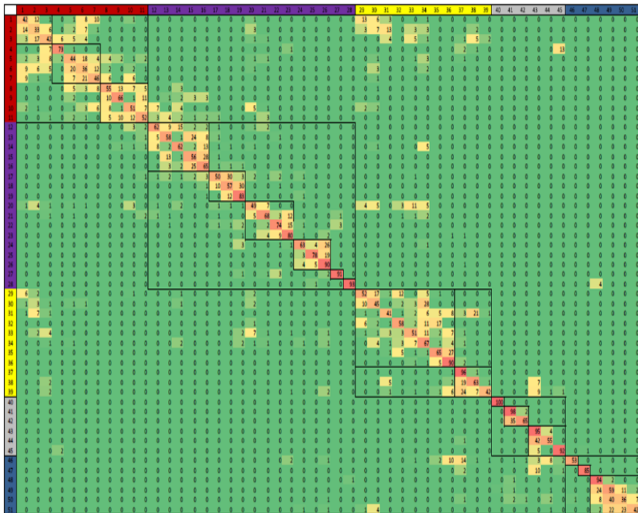
Figure 19.10: Transition probabilities for the final model with 51 states. The transition probability increases from green to red. Spatial relationships between neighboring chromatin states and distinct sub-groups of states are revealed by clustering the transition matrix. Notably, the matrix is sparse, so indicating that most are not possible.
