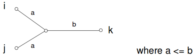
Figure 27.10: Ultrametric distances.
