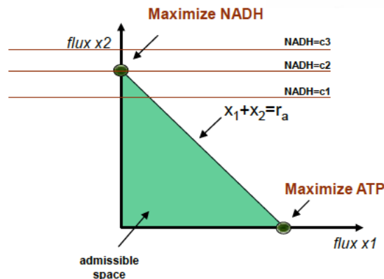
Figure 23.3: Maximizing two functions with linear programming.
