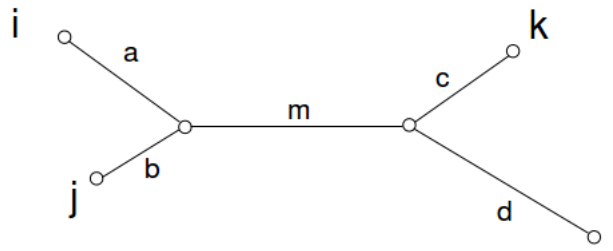
Figure 27.11: Additive distances.
