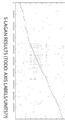
Figure 5.27: S-LAGAN results.
