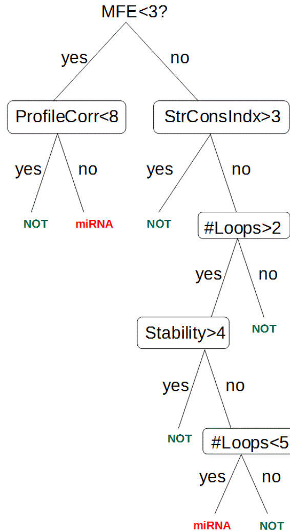
Figure 4.28: A possible decision tree for miRNA detection. The features used in this tree are minimum free energy, conservation profile correlation, structure conservation index, number of loops, and stability.
