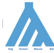
Figure 28.1: Species Tree
