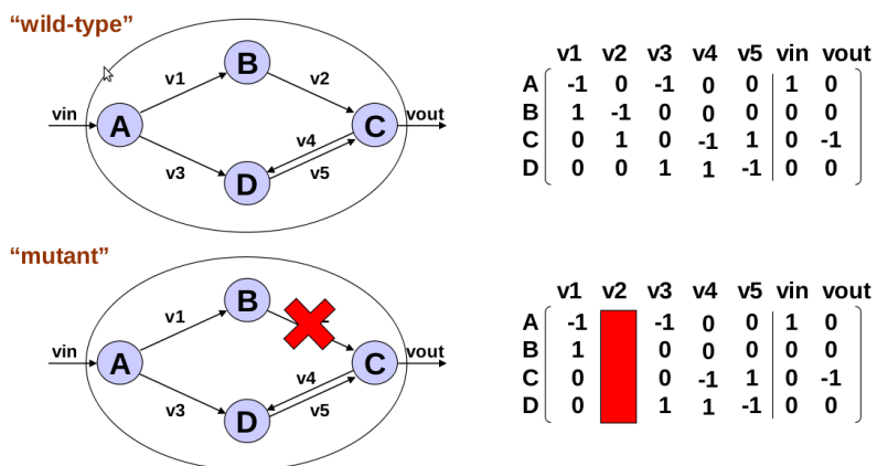
Figure 23.4: Removing a reaction is the same as removing a gene from the stoichiometric matrix.
