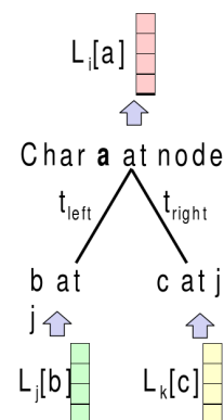
Figure 27.19: The recurrence
