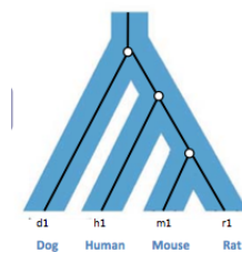
Figure 28.3: Gene Tree Inside a Species Tree
