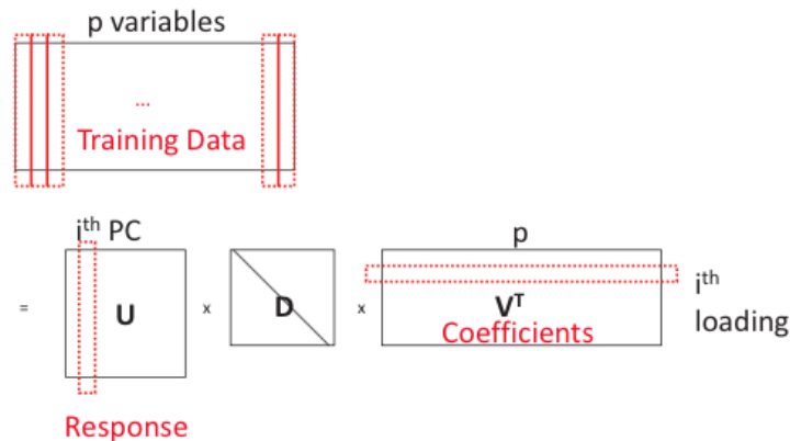
Figure 20.8: PCA in a regression framework
