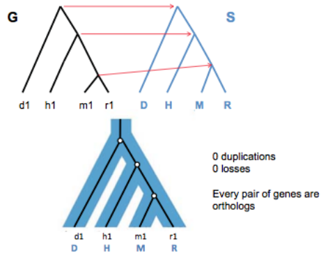
Figure 28.9: Reconciliation Example 1, simple mapping case
