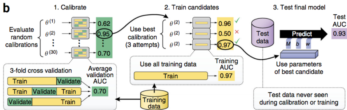
Figure 20.18: An illustration of the calibration, training and testing procedure used by the DeepBind method (taken from the DeepBind paper).
